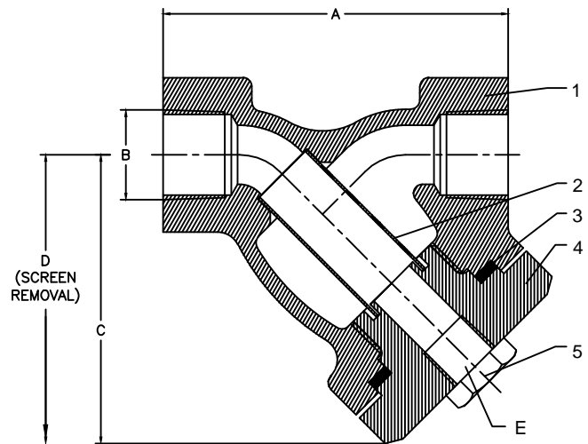
THREADED END
