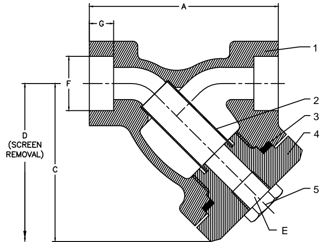
SOCKET WELD END
